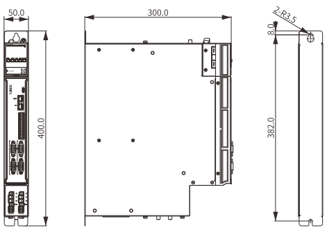
DM6C-40P4/40P7/41P5/43P0-M
