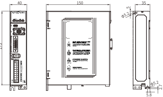
DS6C-20P4
