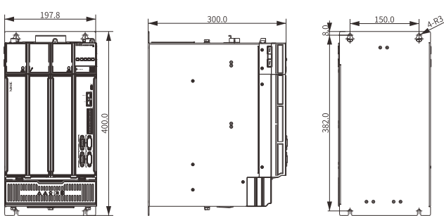
DM6C-445P0/455P0S/475P0S-M
