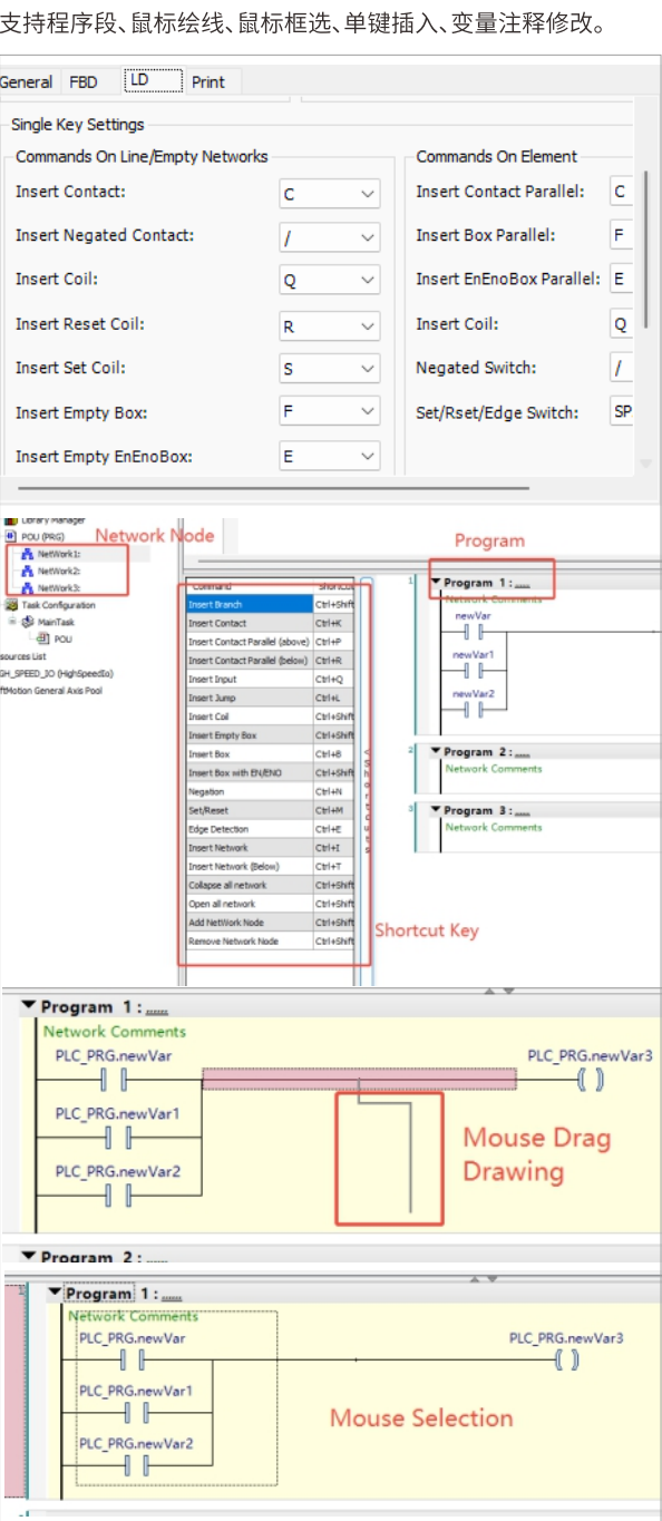
Ladder editor
